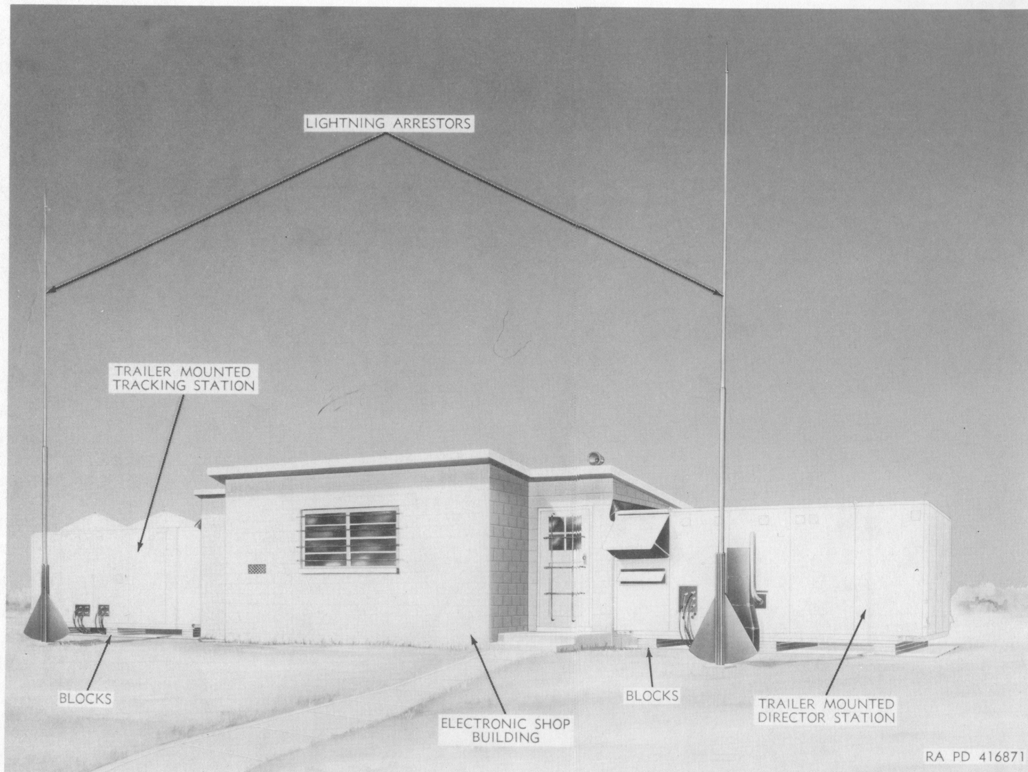
Figure 127. Trailers emplaced, permanent site.
